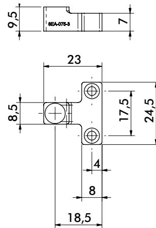
Part Present Sensor Part Number 8EA-075-2 3mm Sensing Distance, 2m Cable 8EA-075-3 3mm Sensing Distance, M12X1
