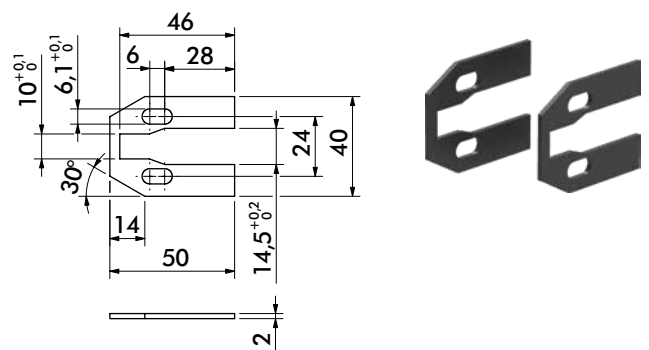
Mount Part Number 8MH-054-1 Guards
