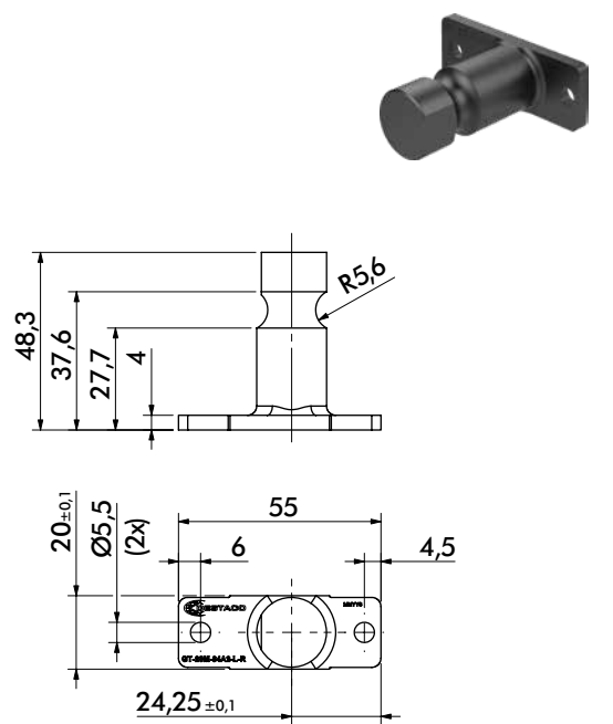
Mount Part Number Ø25mm Rear Rod 8MA-166-1
