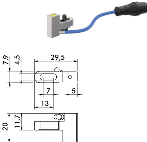
Part Present Sensor Part Number 8EA-087-1 1.5mm Sensing Distance
